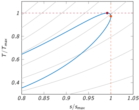
Rayleigh line (Ts-diagram)
