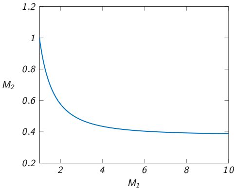
Downstream Mach Number ( \gamma = 1.4 )
