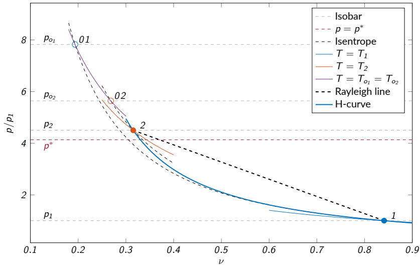
Normal shock ( p\nu -diagram)
